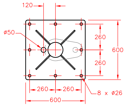
BASE MOUNTING PLAN
